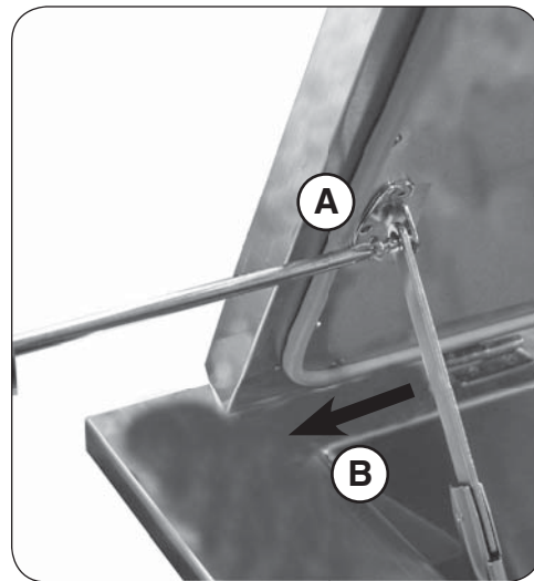
Fig. 2-2 Remove hinges
